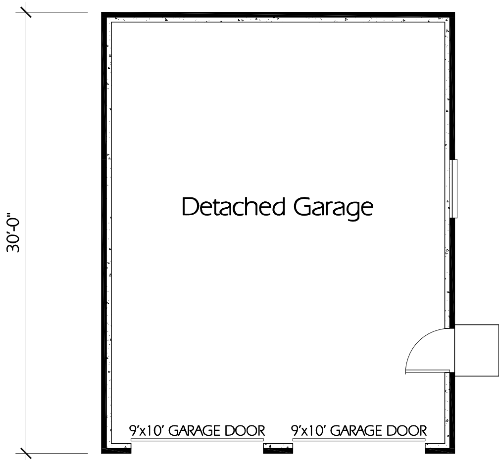
Garage 24'-x30' Version A
